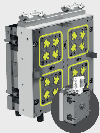
two platen concept
